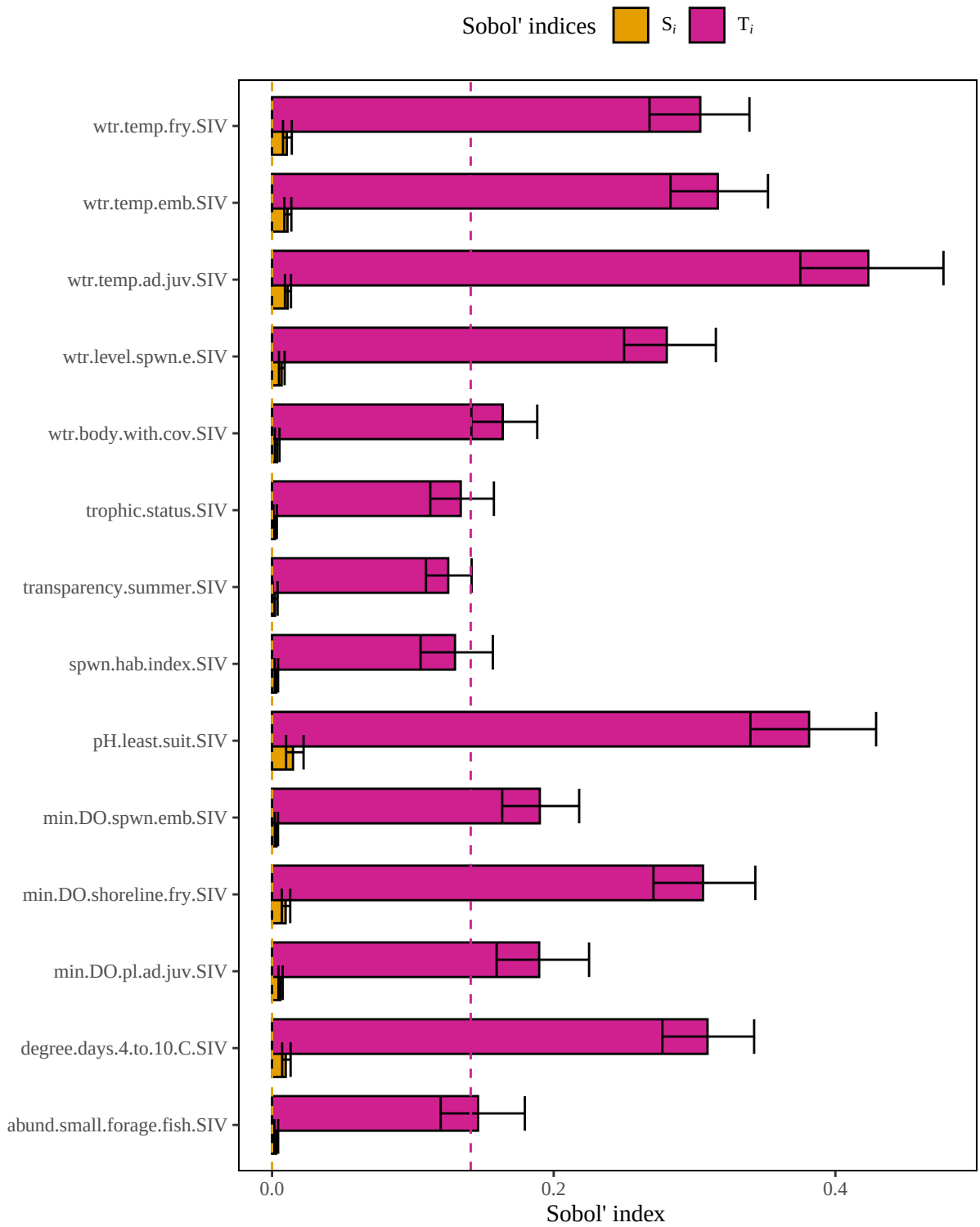
Figure 7. Results of a sensitivity analysis for the walleyeLacSecchiMt3.4m model based on a multiplicative mean structure. Dashed lines represent baseline numerical approximation error for S_i and T_i ( i.e. , dummy variables).
